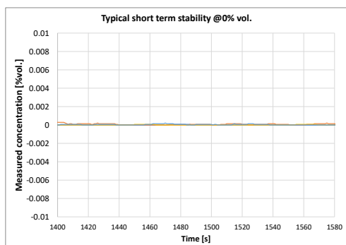
Typical Short Term Precision/Stability @0%
