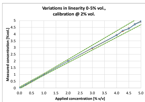
Typical Linearity 0-5%
