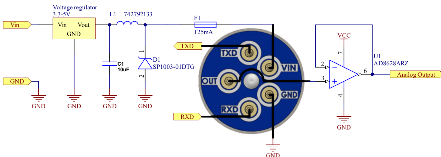
Fig.1 Example schematic for Interfacing Integrated IR (INIR2-CD5PC)
